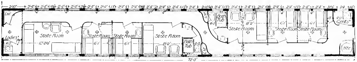
Fig. 176. SECTIONAL PLAN OF COMPARTMENT SLEEPING CAR, SAN SALVADOR.
